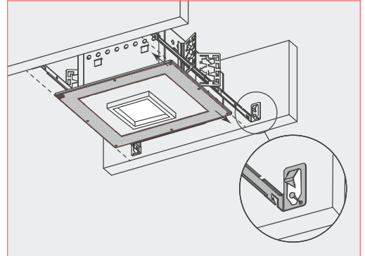
HANGER BAR MOUNTING
