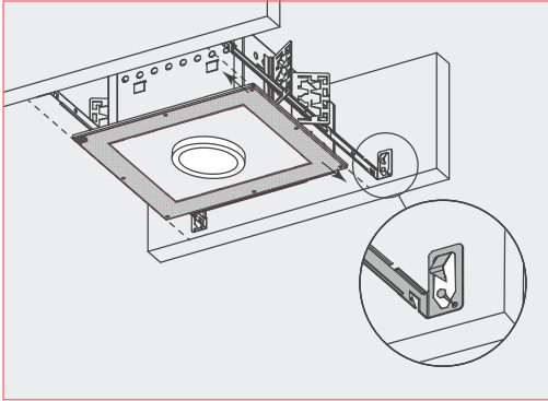
HANGER BAR MOUNTING
