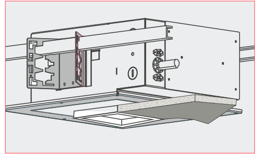
BUTTERFLY BRACKET MOUNTING
