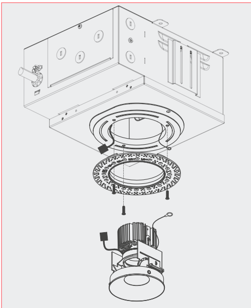
INSTALLATION OF VF100 LAMP MODULE AND TRIM
