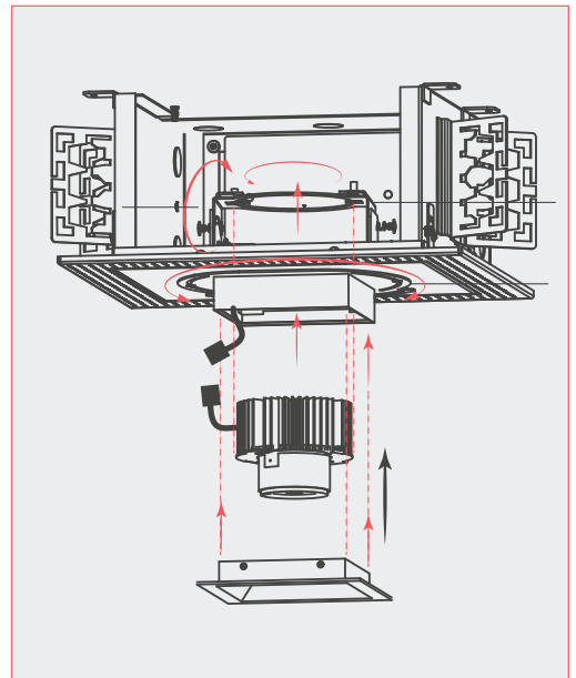
INSTALLATION OF VF150 LAMP MODULE AND TRIM
