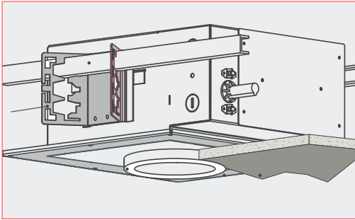
BUTTERFLY BRACKET MOUNTING
