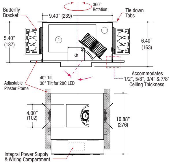
(HVS-1BA-T) SMALL SIZED HOUSING (AD) Adjustable Downlight
