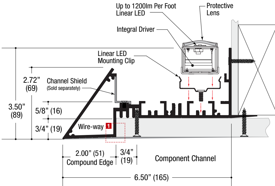
EFK2 CHANNEL PROFILE (Figure 1)
