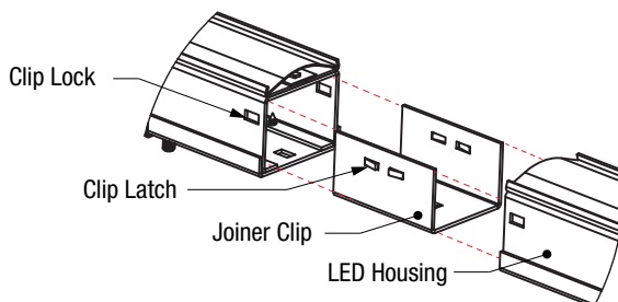
LINEAR LED JOINER CLIP (Figure 3)
