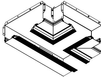
TE 90° 3-Way Connection
