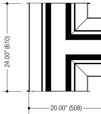
TE 90° 3-Way Connection
