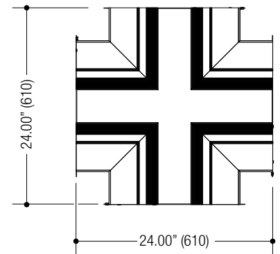
XC 90° 4-Way Connection
