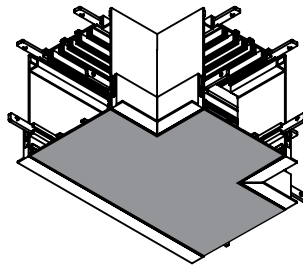
TEE 90° 3-Way Connection
