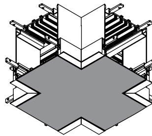
4WY 90° 4-Way Connection
