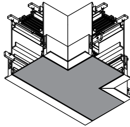
TEE 90° 3-Way Connection
