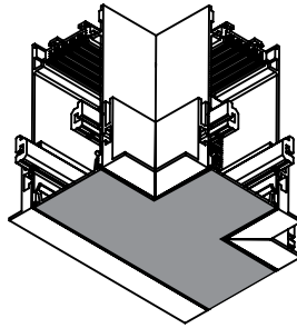
TEE 90° 3-Way Connection
