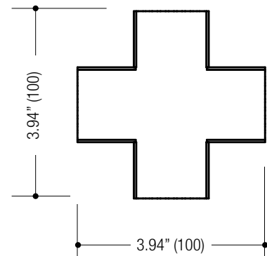
4WY 90° 4-Way Connection
